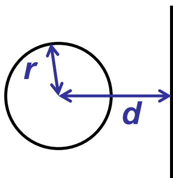
ring torus r < d
