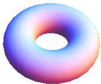
ring torus r < d
