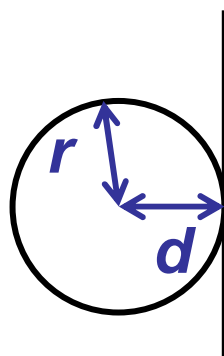
horn torus r = d
